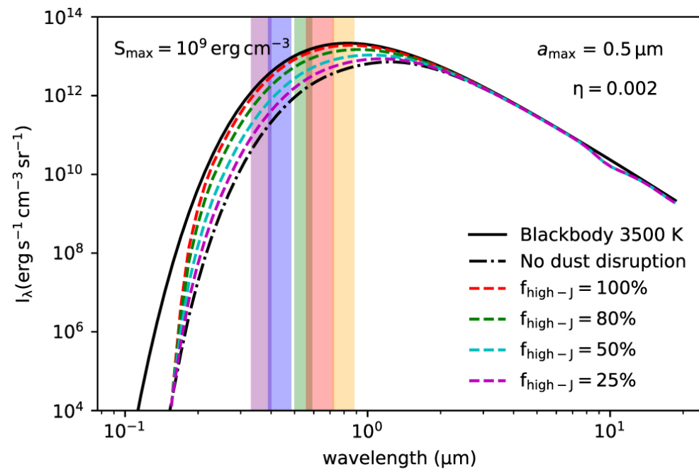
Figure 14. from Bao Truong et al 2022 Astrophys. J. 936 doi:10.3847/1538-4357/ac86d9 https://dx.doi.org/10.3847/1538-4357/ac86d9 © 2022. The Author(s). Published by the American Astronomical Society.
