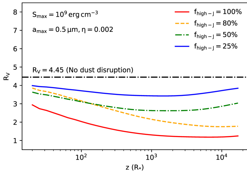
Figure 11. from Bao Truong et al 2022 Astrophys. J. 936 doi:10.3847/1538-4357/ac86d9 https://dx.doi.org/10.3847/1538-4357/ac86d9 © 2022. The Author(s). Published by the American Astronomical Society.
