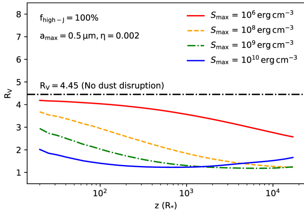
Figure 10. from Bao Truong et al 2022 Astrophys. J. 936 doi:10.3847/1538-4357/ac86d9 https://dx.doi.org/10.3847/1538-4357/ac86d9 © 2022. The Author(s). Published by the American Astronomical Society.
