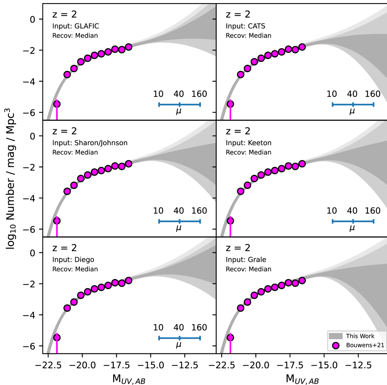
Figure 14. from R. J. Bouwens et al 2022 Astrophys. J. 940 doi:10.3847/1538-4357/ac86d1 https://dx.doi.org/10.3847/1538-4357/ac86d1 © 2022. The Author(s). Published by the American Astronomical Society.
