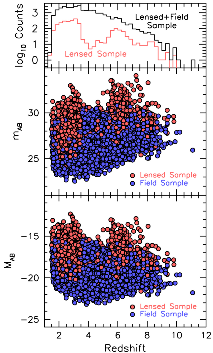
Figure 1. from R. J. Bouwens et al 2022 Astrophys. J. 940 doi:10.3847/1538-4357/ac86d1 https://dx.doi.org/10.3847/1538-4357/ac86d1 © 2022. The Author(s). Published by the American Astronomical Society.
