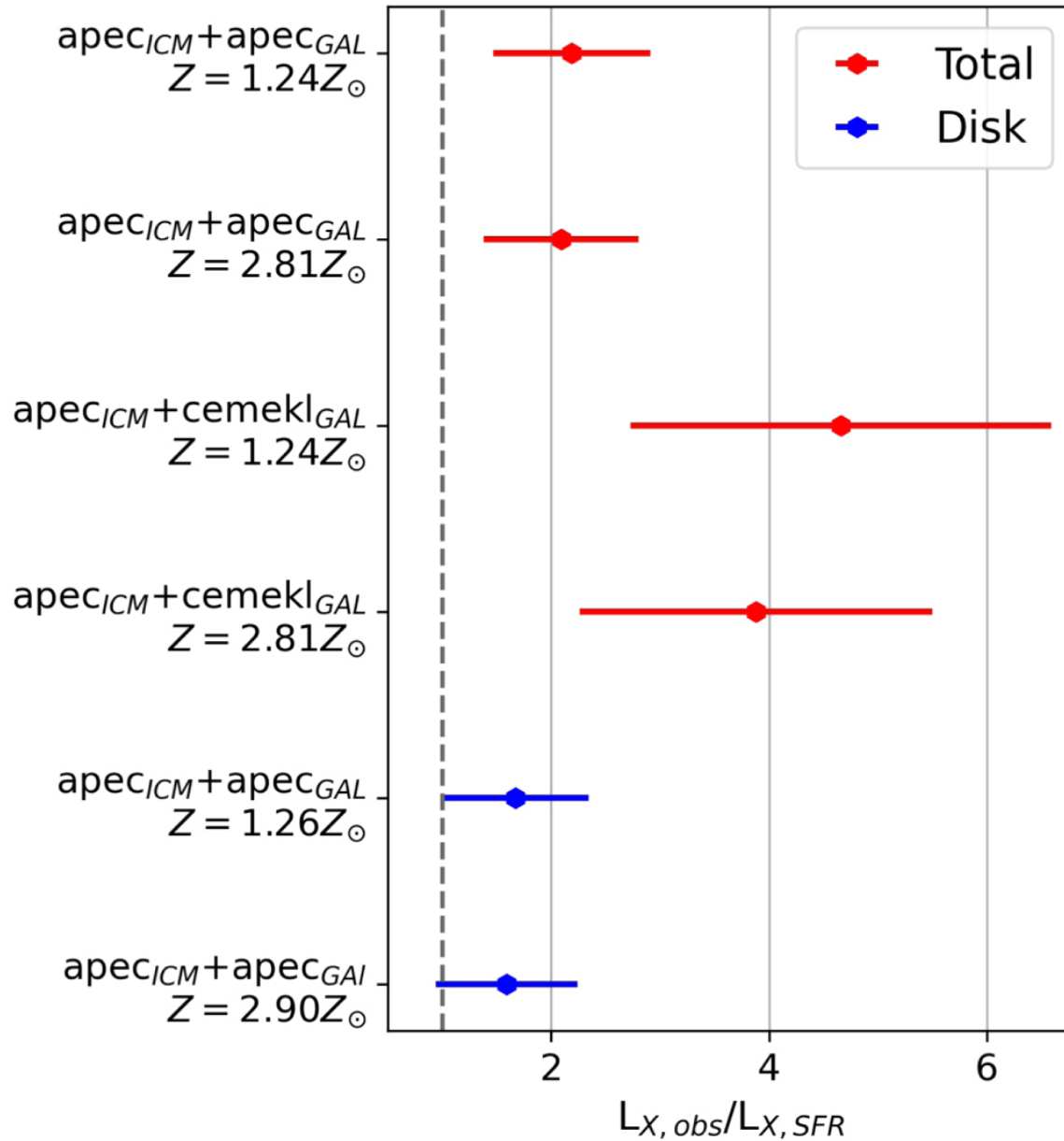
Figure 5. from Chiara Bartolini et al 2022 Astrophys. J. 936 doi:10.3847/1538-4357/ac866a https://dx.doi.org/10.3847/1538-4357/ac866a © 2022. The Author(s). Published by the American Astronomical Society.
