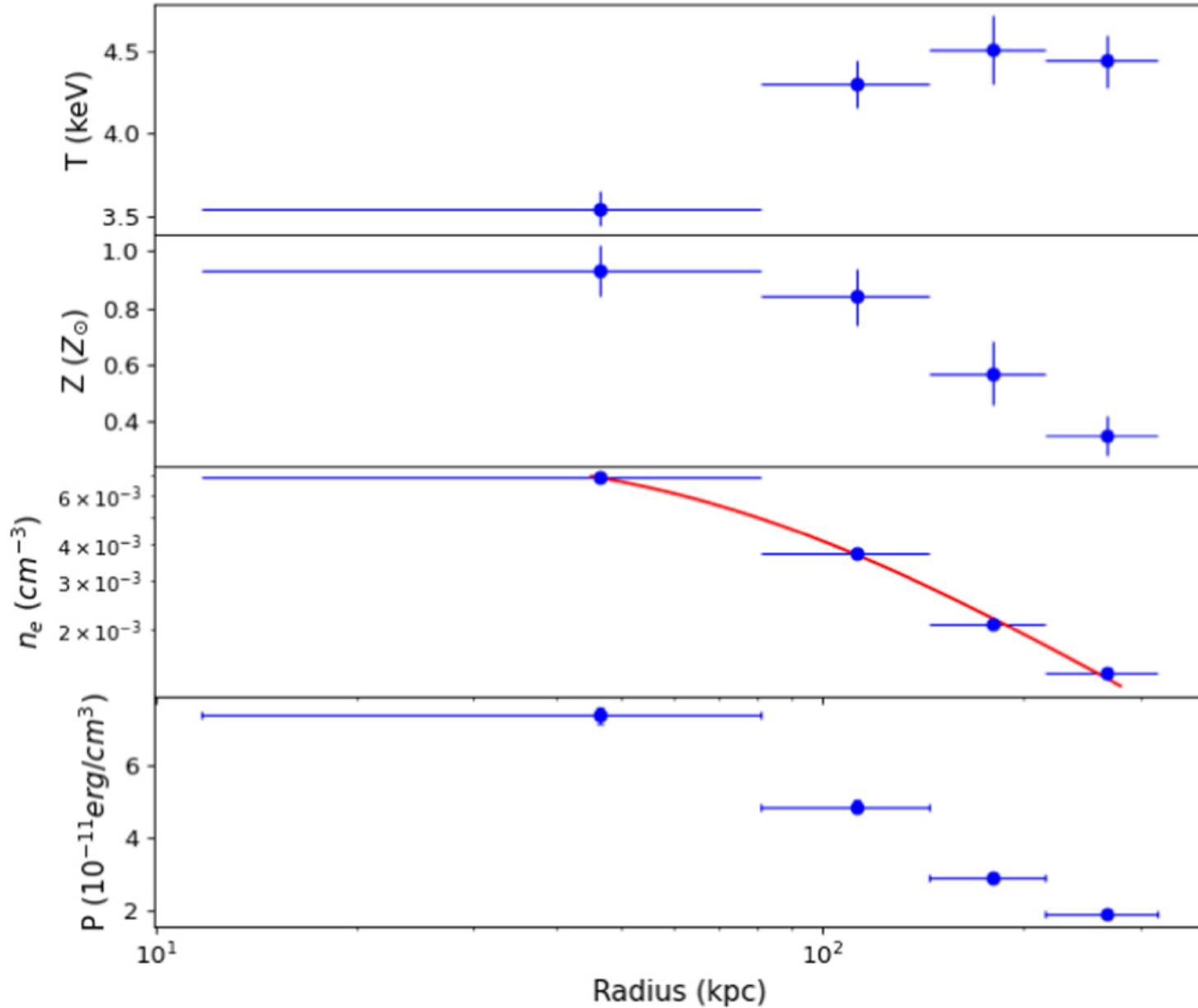
Figure 4. from Chiara Bartolini et al 2022 Astrophys. J. 936 doi:10.3847/1538-4357/ac866a https://dx.doi.org/10.3847/1538-4357/ac866a © 2022. The Author(s). Published by the American Astronomical Society.
