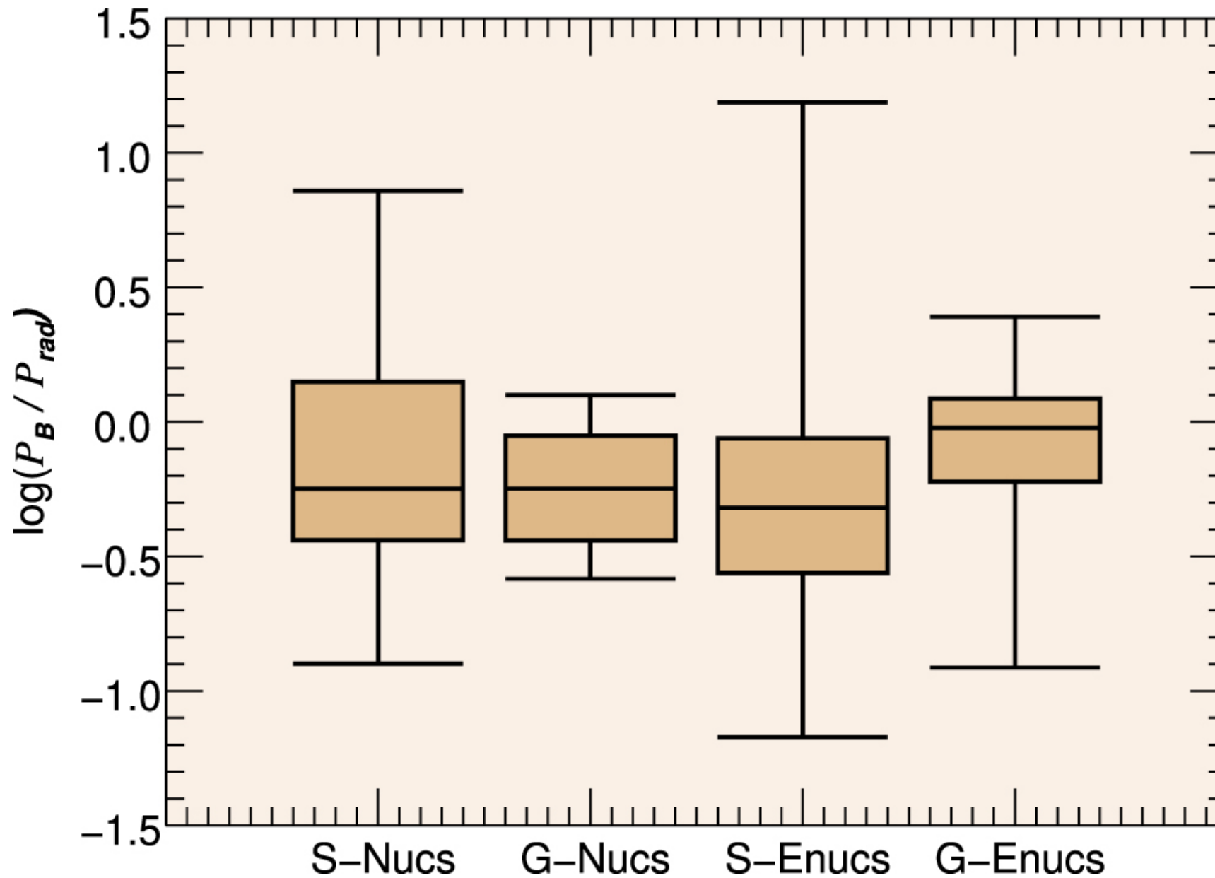
Figure 7. from Eric J. Murphy 2022 Astrophys. J. 938 doi:10.3847/1538-4357/ac8661 https://dx.doi.org/10.3847/1538-4357/ac8661 © 2022. The Author(s). Published by the American Astronomical Society.
