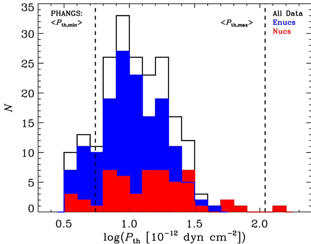
Figure 3. from Eric J. Murphy 2022 Astrophys. J. 938 doi:10.3847/1538-4357/ac8661 https://dx.doi.org/10.3847/1538-4357/ac8661 © 2022. The Author(s). Published by the American Astronomical Society.
