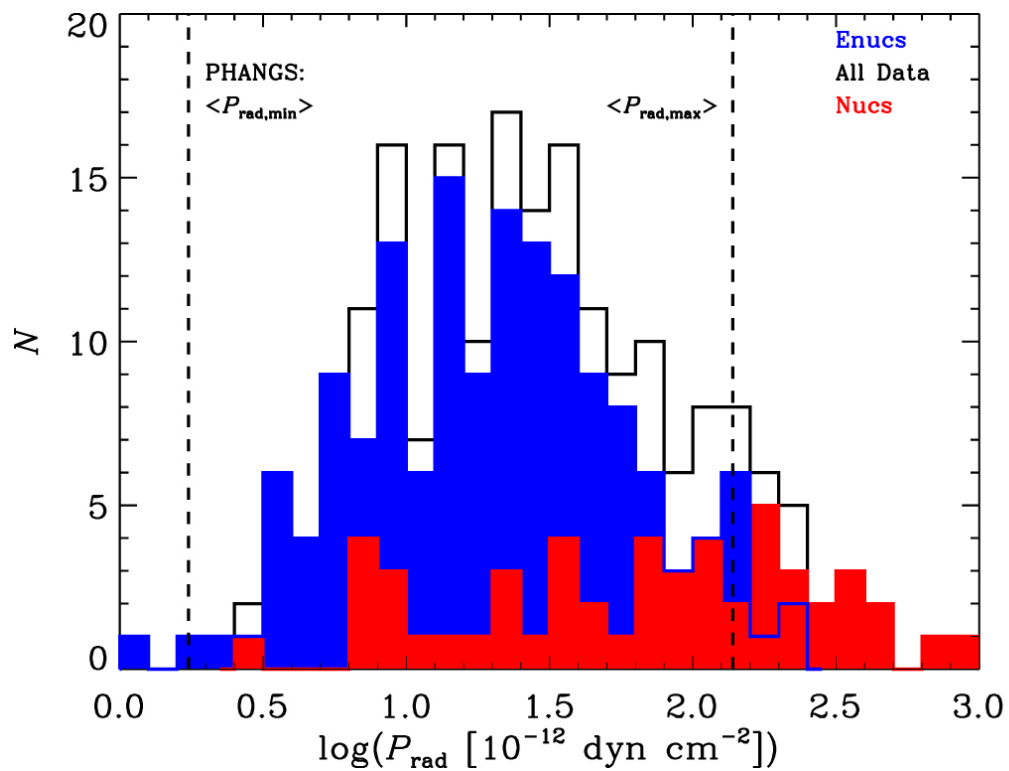
Figure 2. from Eric J. Murphy 2022 Astrophys. J. 938 doi:10.3847/1538-4357/ac8661 https://dx.doi.org/10.3847/1538-4357/ac8661 © 2022. The Author(s). Published by the American Astronomical Society.
