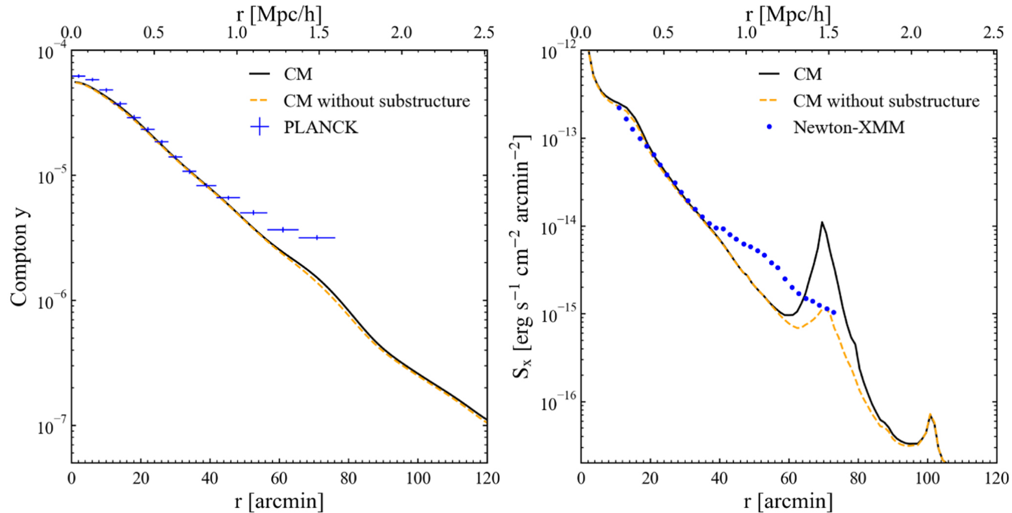
Figure 9. from Renjie Li et al 2022 Astrophys. J. 936 doi:10.3847/1538-4357/ac8359 https://dx.doi.org/10.3847/1538-4357/ac8359 © 2022. The Author(s). Published by the American Astronomical Society.
