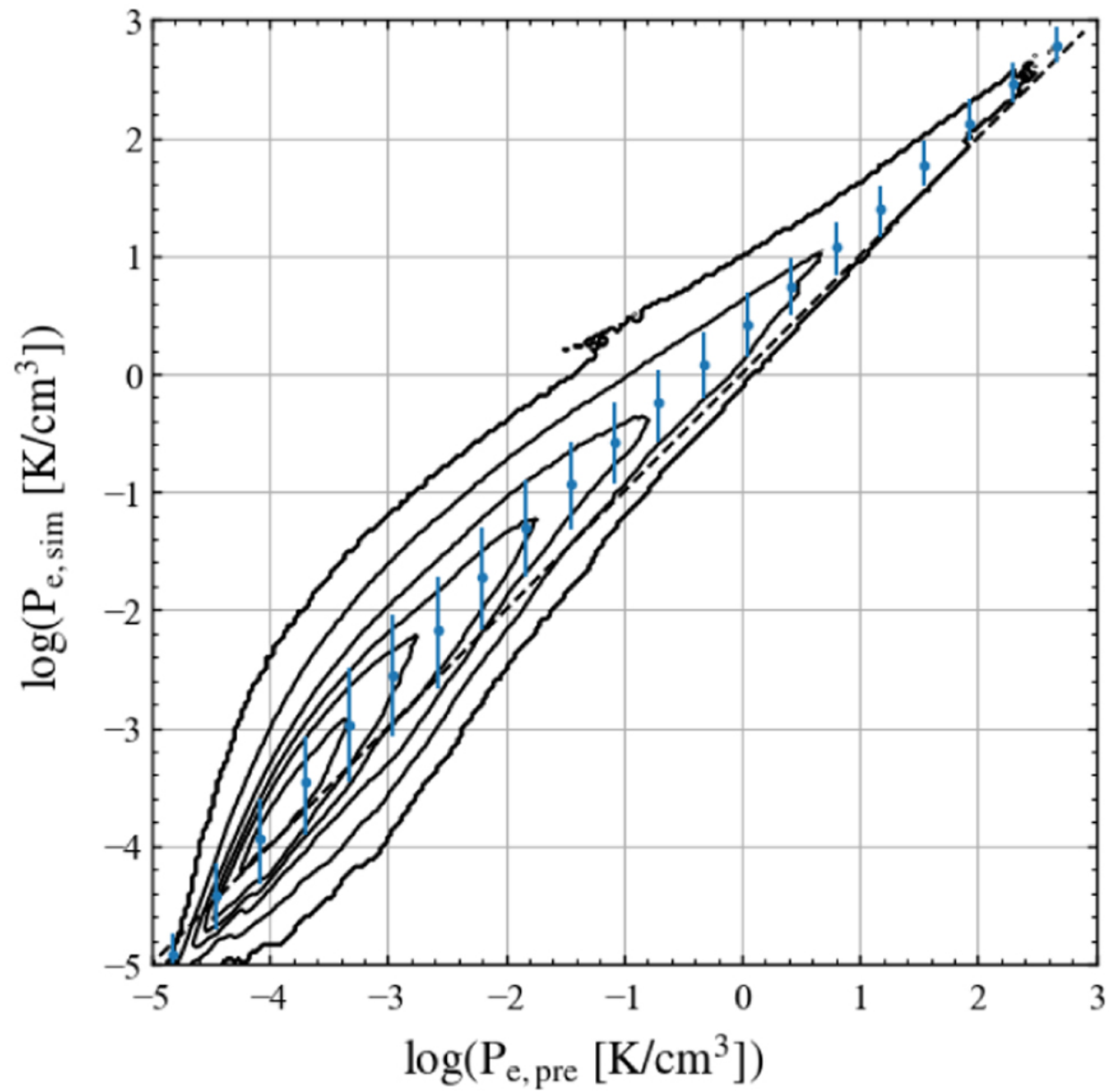
Figure 8. from Renjie Li et al 2022 Astrophys. J. 936 doi:10.3847/1538-4357/ac8359 https://dx.doi.org/10.3847/1538-4357/ac8359 © 2022. The Author(s). Published by the American Astronomical Society.
