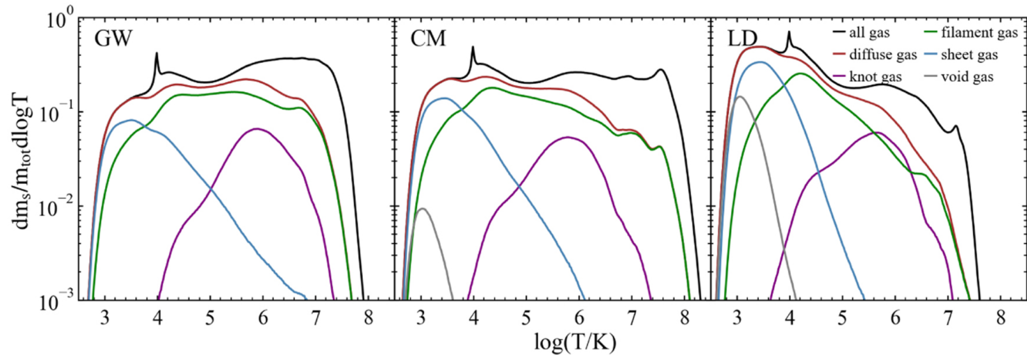
Figure 5. from Renjie Li et al 2022 Astrophys. J. 936 doi:10.3847/1538-4357/ac8359 https://dx.doi.org/10.3847/1538-4357/ac8359 © 2022. The Author(s). Published by the American Astronomical Society.
