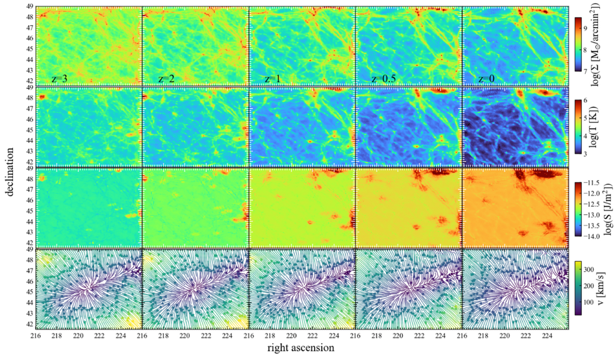
Figure 4. from Renjie Li et al 2022 Astrophys. J. 936 doi:10.3847/1538-4357/ac8359 https://dx.doi.org/10.3847/1538-4357/ac8359 © 2022. The Author(s). Published by the American Astronomical Society.
