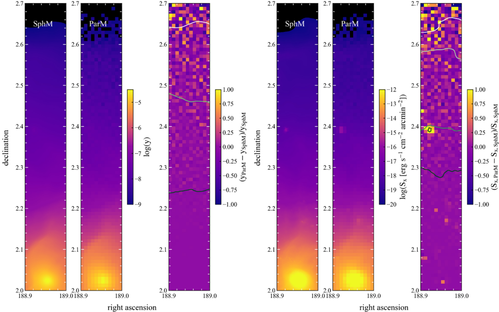
Figure 14. from Renjie Li et al 2022 Astrophys. J. 936 doi:10.3847/1538-4357/ac8359 https://dx.doi.org/10.3847/1538-4357/ac8359 © 2022. The Author(s). Published by the American Astronomical Society.
