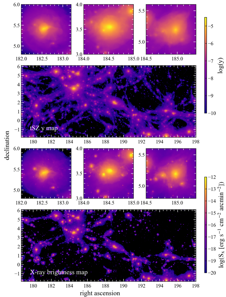
Figure 11. from Renjie Li et al 2022 Astrophys. J. 936 doi:10.3847/1538-4357/ac8359 https://dx.doi.org/10.3847/1538-4357/ac8359 © 2022. The Author(s). Published by the American Astronomical Society.
