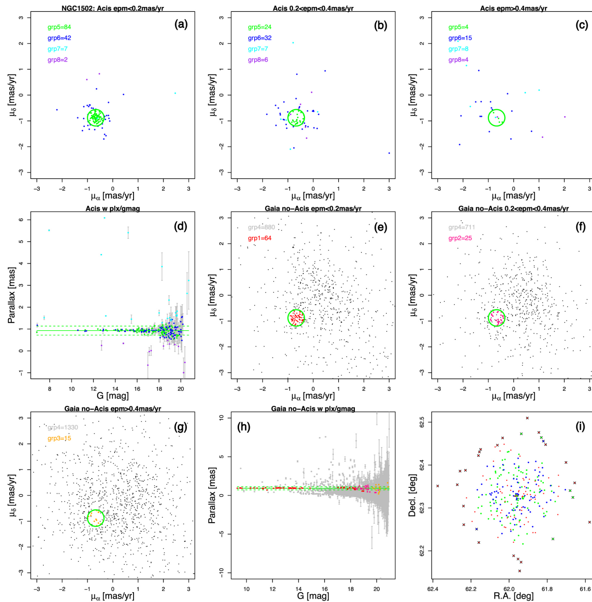
Figure 2. Astrometry for X-ray and non-X-ray sources from Konstantin V. Getman et al 2022 Astrophys. J. 935 doi:10.3847/1538-4357/ac7c69 https://dx.doi.org/10.3847/1538-4357/ac7c69
