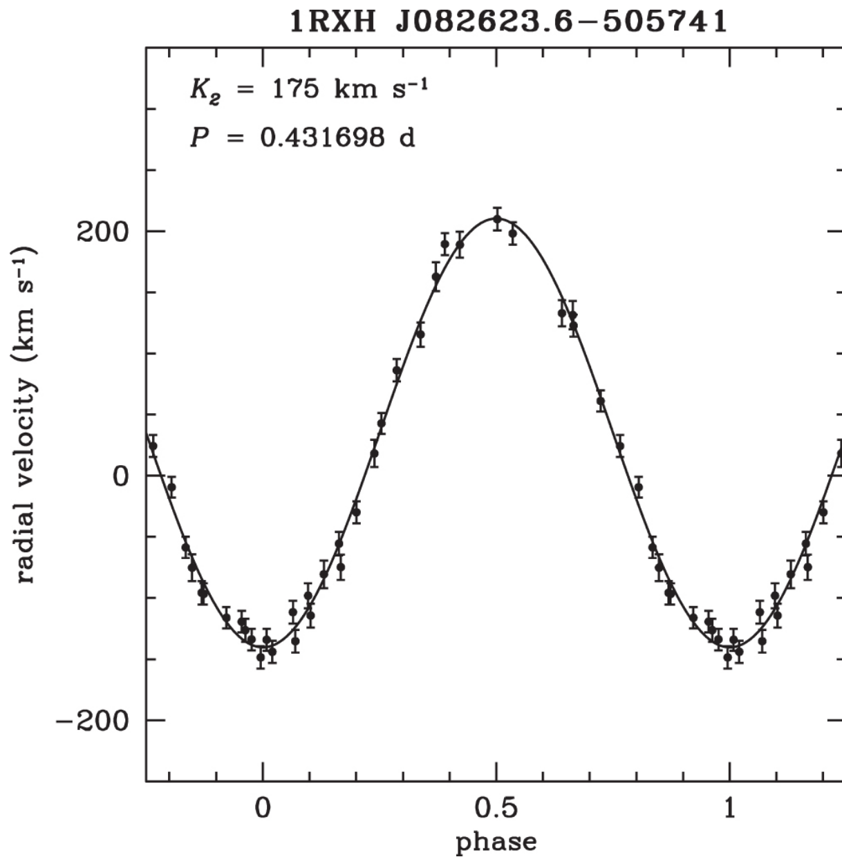
Figure 8. from Kirill V. Sokolovsky et al 2022 Astrophys. J. 934 doi:10.3847/1538-4357/ac7b25 https://dx.doi.org/10.3847/1538-4357/ac7b25 © 2022. The Author(s). Published by the American Astronomical Society.
