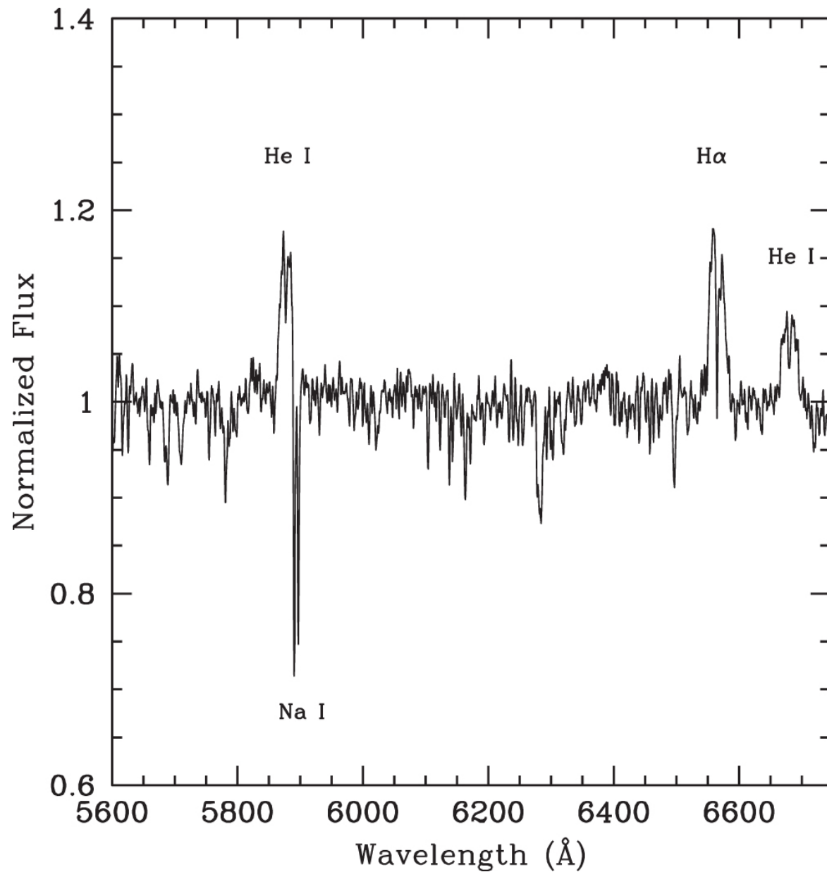
Figure 7. from Kirill V. Sokolovsky et al 2022 Astrophys. J. 934 doi:10.3847/1538-4357/ac7b25 https://dx.doi.org/10.3847/1538-4357/ac7b25 © 2022. The Author(s). Published by the American Astronomical Society.
