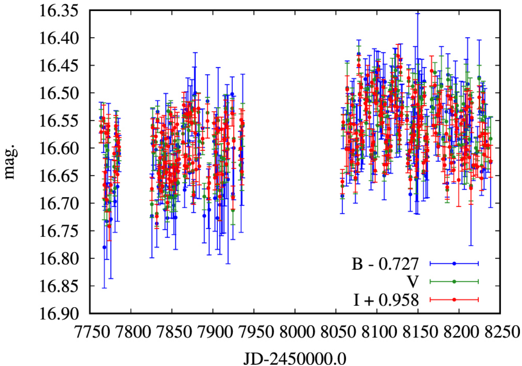
Figure 5. from Kirill V. Sokolovsky et al 2022 Astrophys. J. 934 doi:10.3847/1538-4357/ac7b25 https://dx.doi.org/10.3847/1538-4357/ac7b25 © 2022. The Author(s). Published by the American Astronomical Society.
