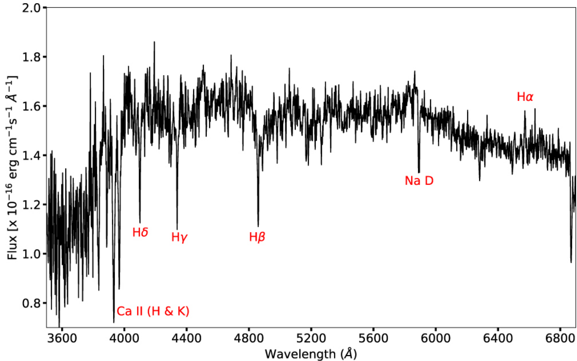
Figure 4. from Kirill V. Sokolovsky et al 2022 Astrophys. J. 934 doi:10.3847/1538-4357/ac7b25 https://dx.doi.org/10.3847/1538-4357/ac7b25 © 2022. The Author(s). Published by the American Astronomical Society.
