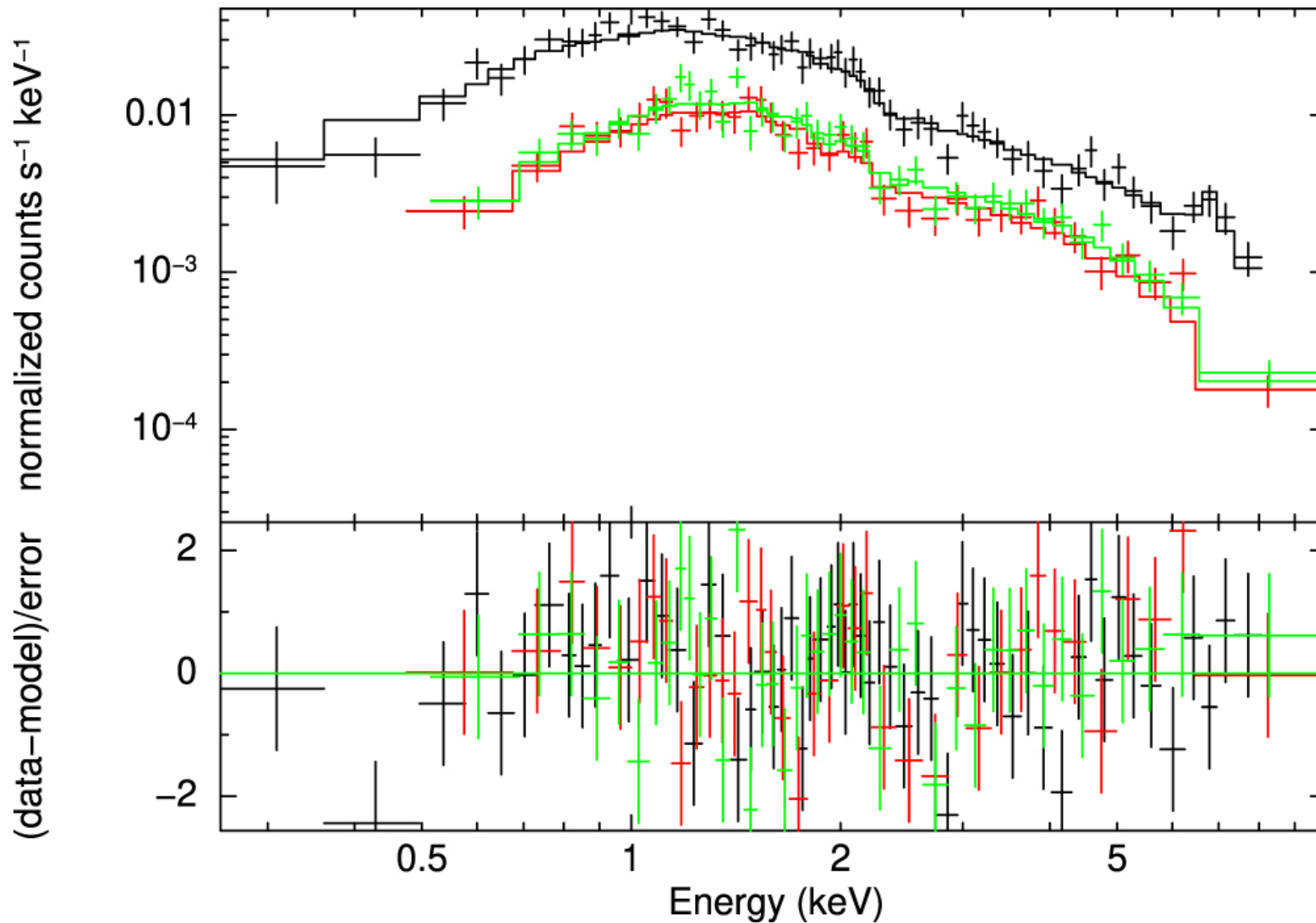
Figure 2. from Kirill V. Sokolovsky et al 2022 Astrophys. J. 934 doi:10.3847/1538-4357/ac7b25 https://dx.doi.org/10.3847/1538-4357/ac7b25 © 2022. The Author(s). Published by the American Astronomical Society.
