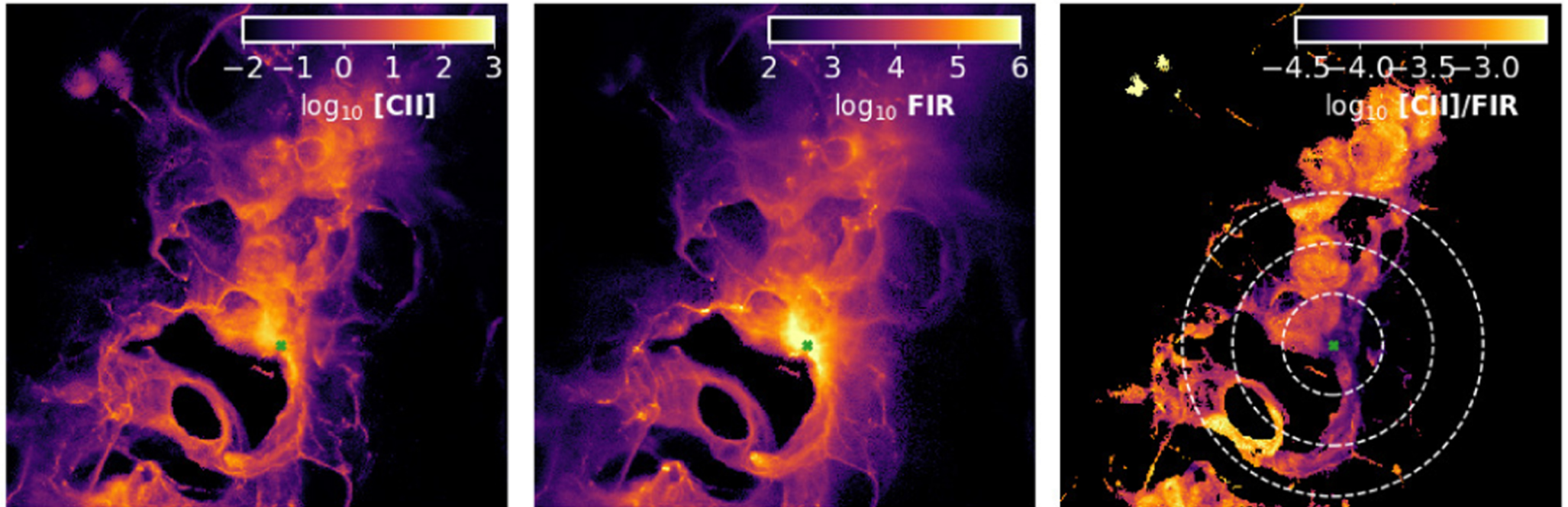
Figure 9. from Thomas G. Bisbas et al 2022 Astrophys. J. 934 doi:10.3847/1538-4357/ac7960 https://dx.doi.org/10.3847/1538-4357/ac7960 © 2022. The Author(s). Published by the American Astronomical Society.
