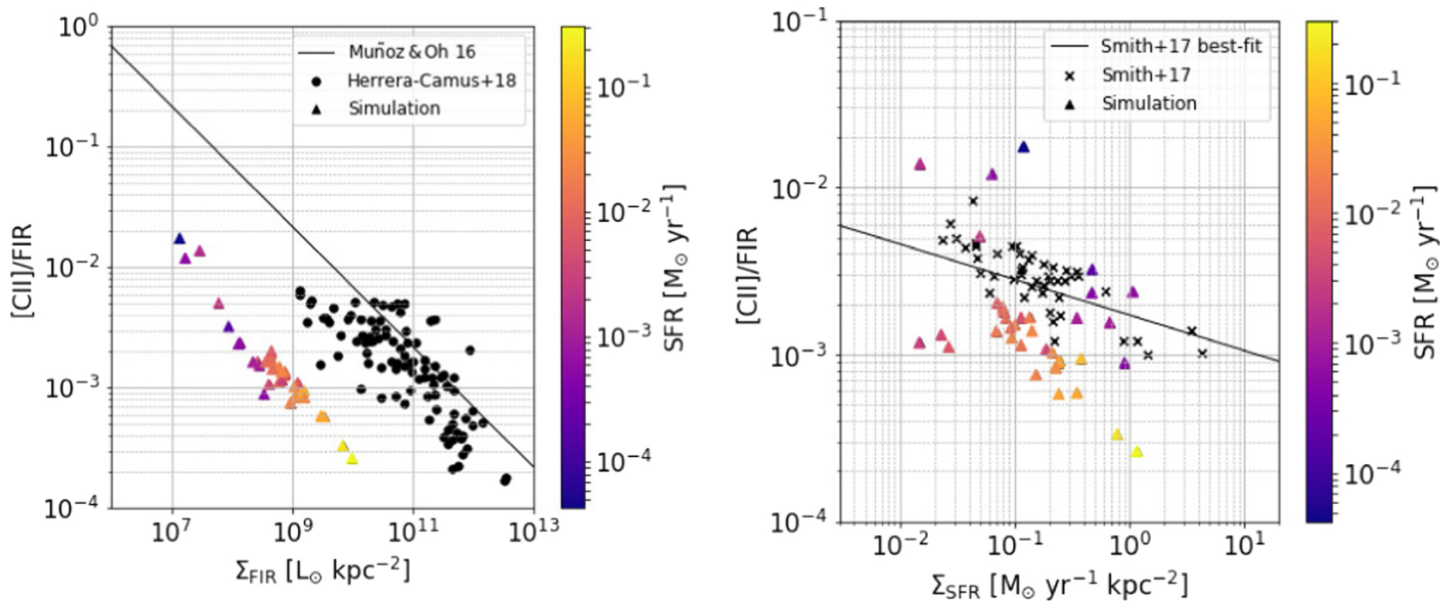
Figure 8. from Thomas G. Bisbas et al 2022 Astrophys. J. 934 doi:10.3847/1538-4357/ac7960 https://dx.doi.org/10.3847/1538-4357/ac7960 © 2022. The Author(s). Published by the American Astronomical Society.
