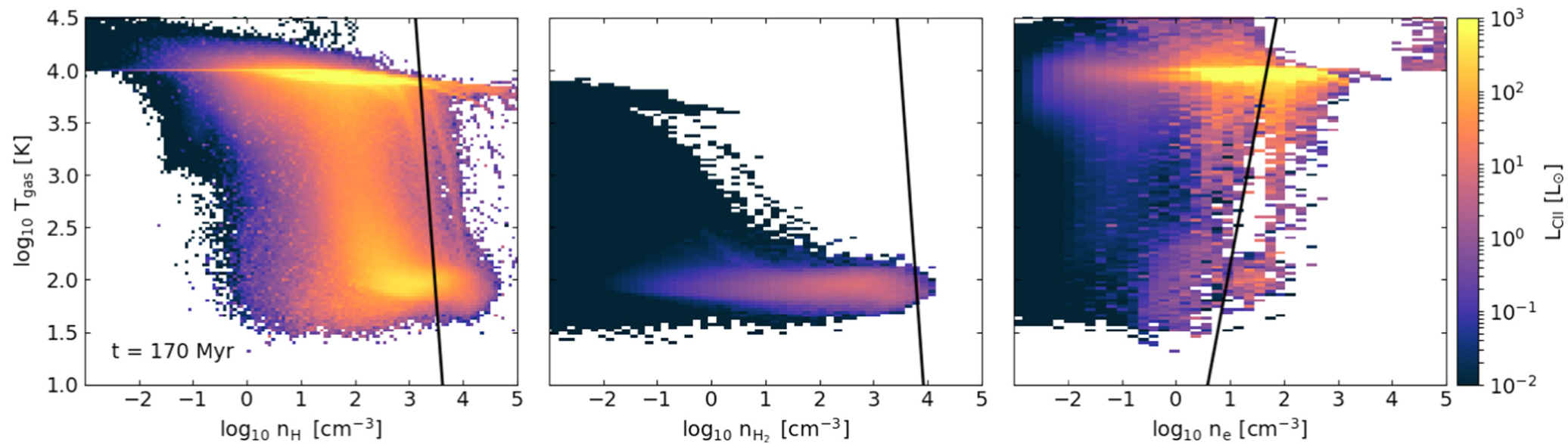
Figure 6. from Thomas G. Bisbas et al 2022 Astrophys. J. 934 doi:10.3847/1538-4357/ac7960 https://dx.doi.org/10.3847/1538-4357/ac7960 © 2022. The Author(s). Published by the American Astronomical Society.
