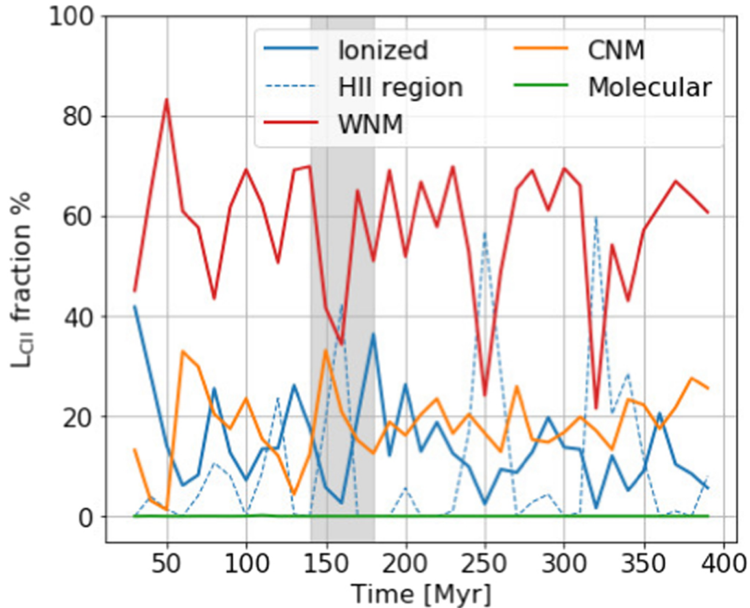
Figure 4. from Thomas G. Bisbas et al 2022 Astrophys. J. 934 doi:10.3847/1538-4357/ac7960 https://dx.doi.org/10.3847/1538-4357/ac7960 © 2022. The Author(s). Published by the American Astronomical Society.
