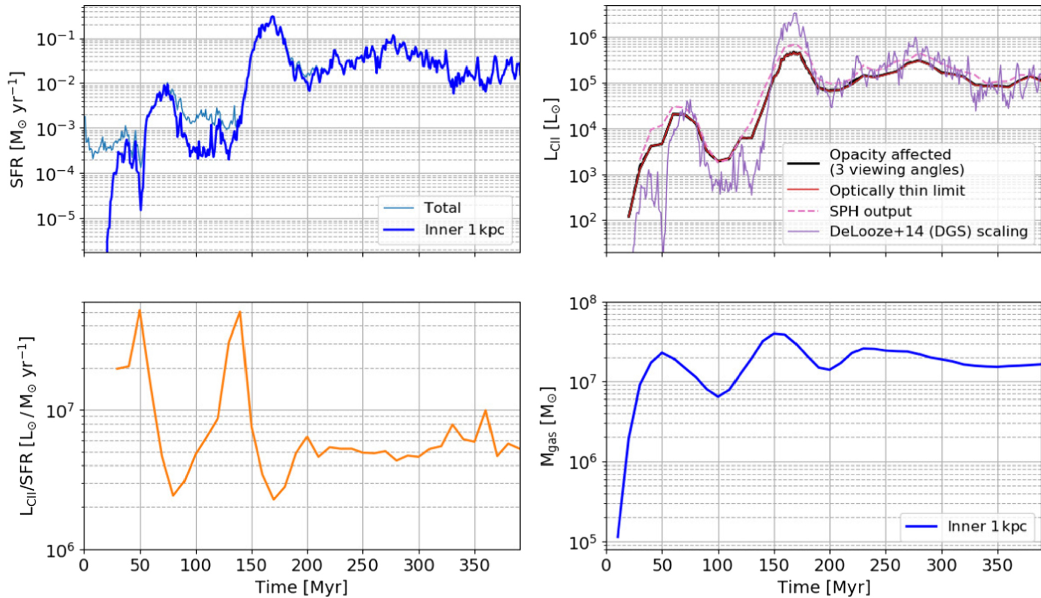
Figure 2. from Thomas G. Bisbas et al 2022 Astrophys. J. 934 doi:10.3847/1538-4357/ac7960 https://dx.doi.org/10.3847/1538-4357/ac7960 © 2022. The Author(s). Published by the American Astronomical Society.
