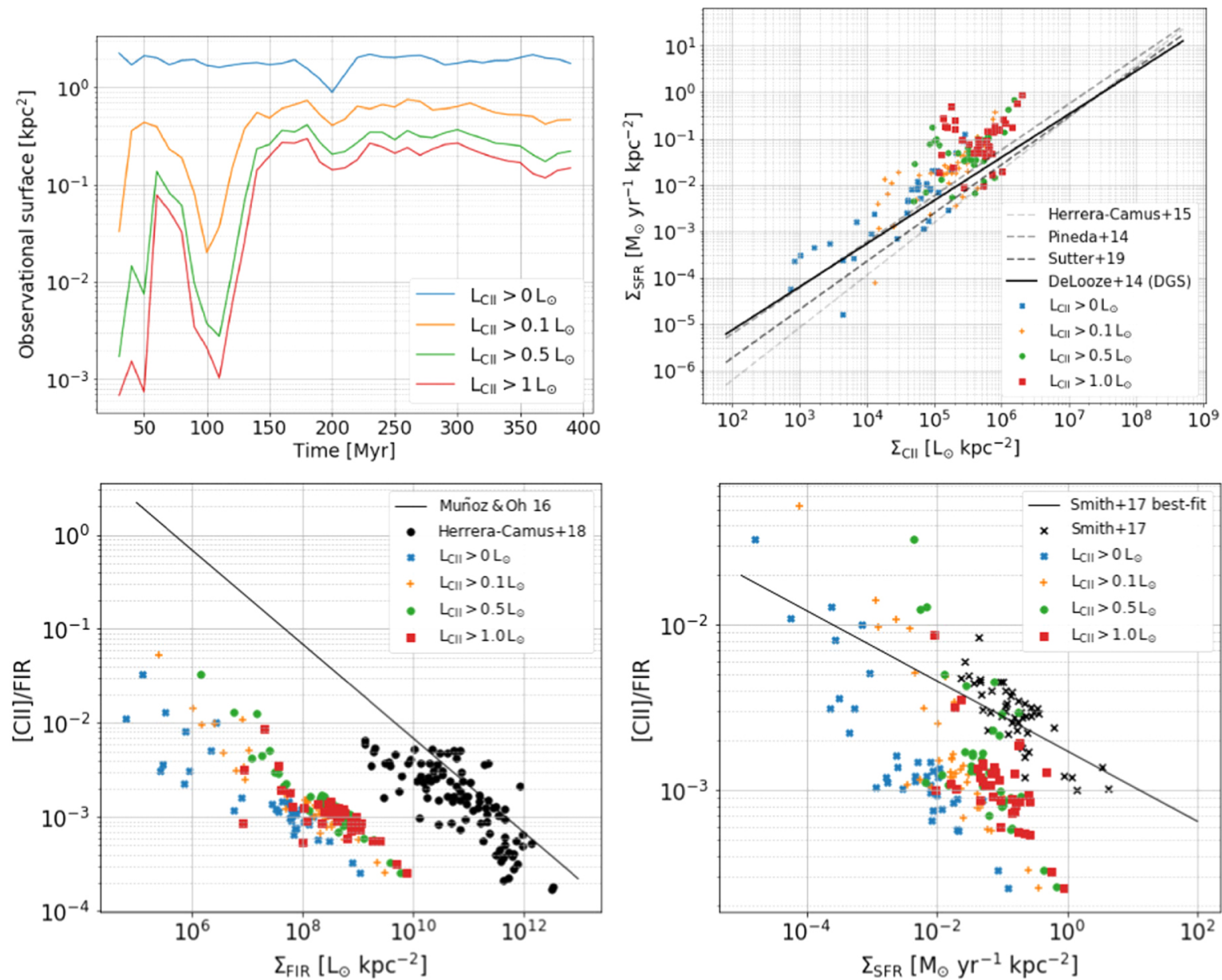
Figure 17. from Thomas G. Bisbas et al 2022 Astrophys. J. 934 doi:10.3847/1538-4357/ac7960 https://dx.doi.org/10.3847/1538-4357/ac7960 © 2022. The Author(s). Published by the American Astronomical Society.
