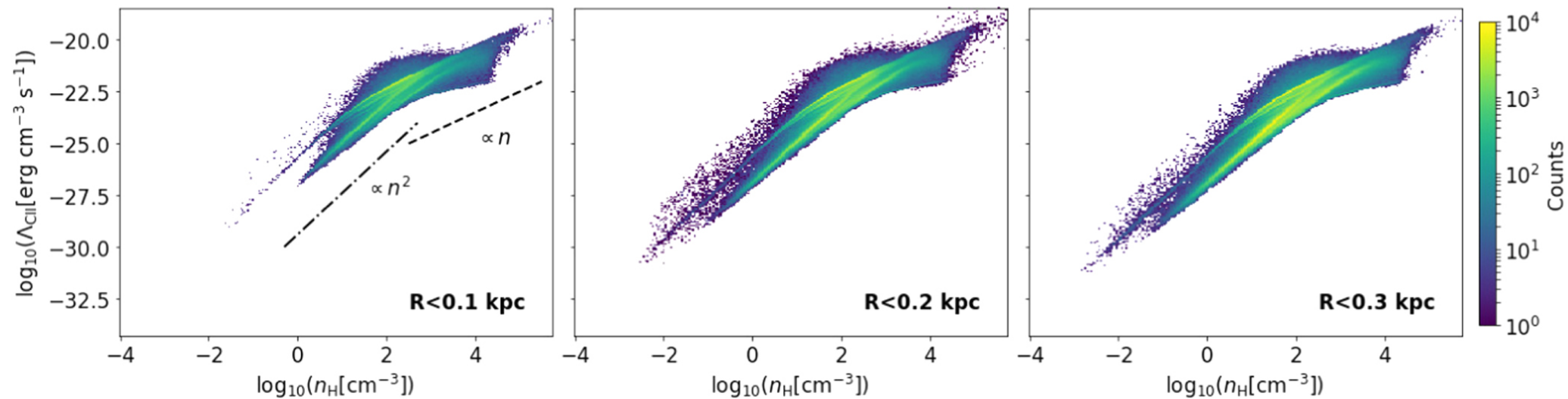
Figure 16. from Thomas G. Bisbas et al 2022 Astrophys. J. 934 doi:10.3847/1538-4357/ac7960 https://dx.doi.org/10.3847/1538-4357/ac7960 © 2022. The Author(s). Published by the American Astronomical Society.
