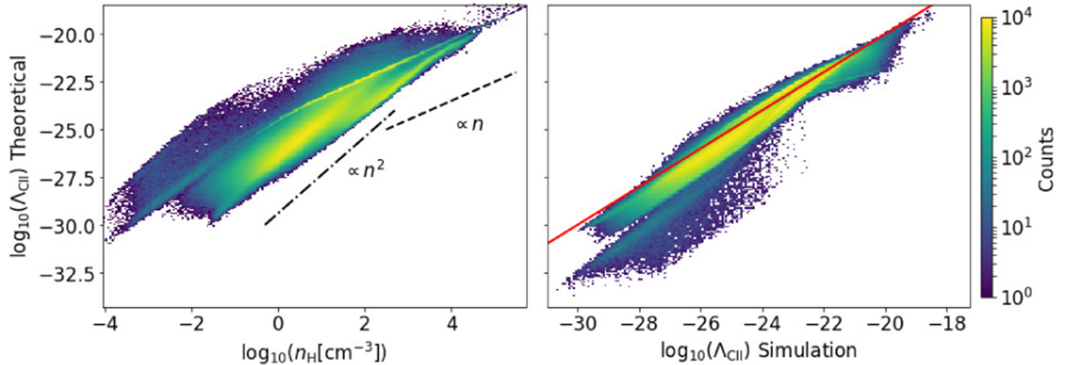
Figure 15. from Thomas G. Bisbas et al 2022 Astrophys. J. 934 doi:10.3847/1538-4357/ac7960 https://dx.doi.org/10.3847/1538-4357/ac7960 © 2022. The Author(s). Published by the American Astronomical Society.
