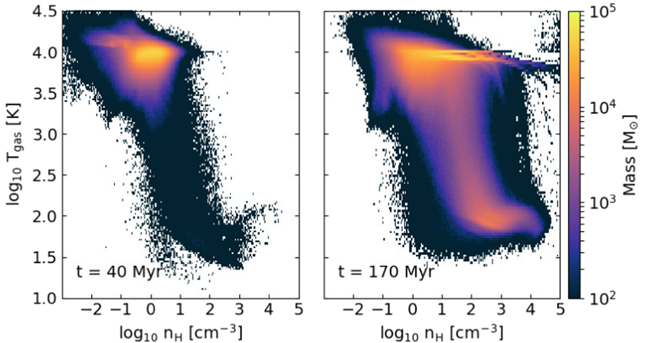
Figure 14. from Thomas G. Bisbas et al 2022 Astrophys. J. 934 doi:10.3847/1538-4357/ac7960 https://dx.doi.org/10.3847/1538-4357/ac7960 © 2022. The Author(s). Published by the American Astronomical Society.
