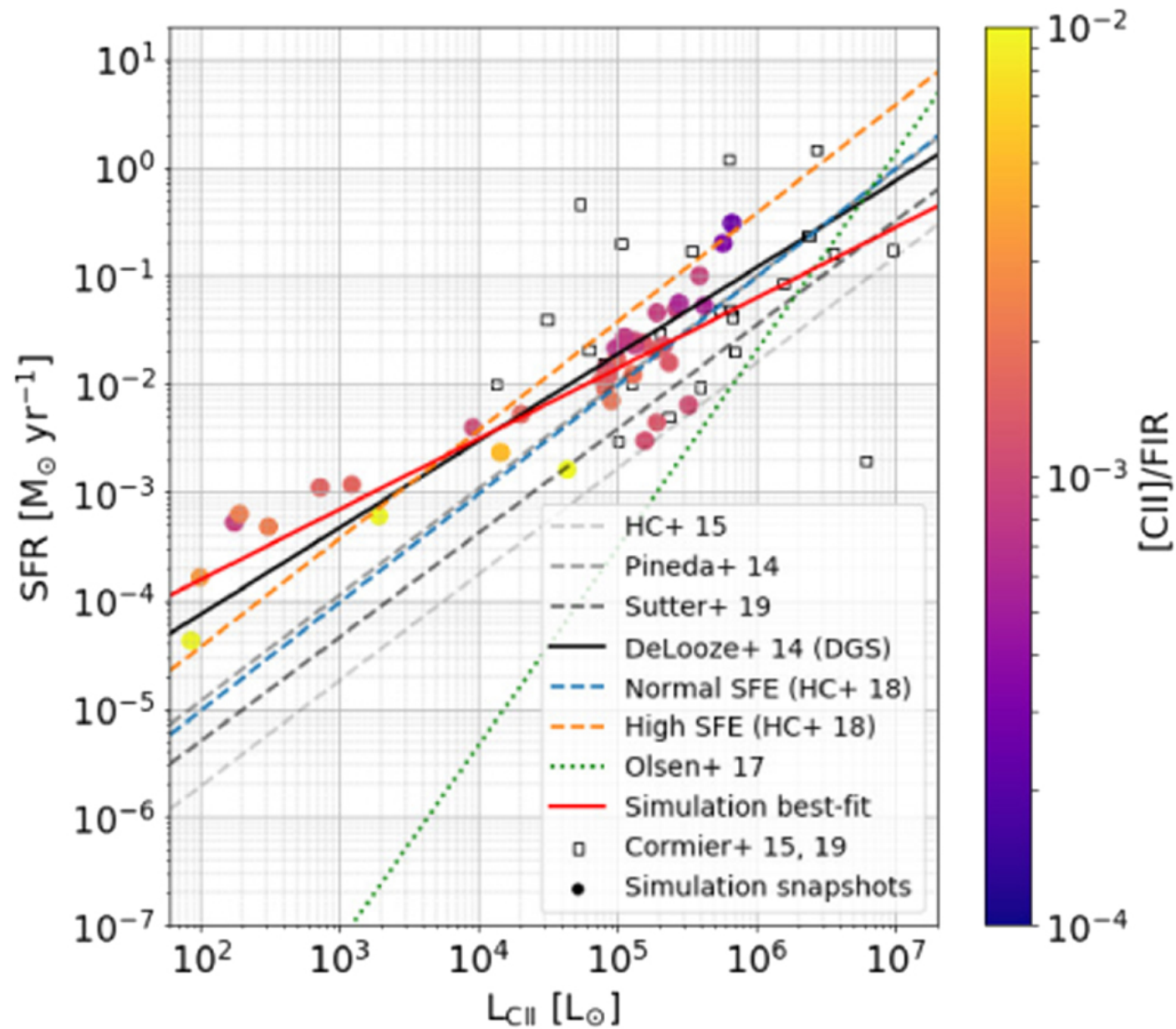
Figure 13. from Thomas G. Bisbas et al 2022 Astrophys. J. 934 doi:10.3847/1538-4357/ac7960 https://dx.doi.org/10.3847/1538-4357/ac7960 © 2022. The Author(s). Published by the American Astronomical Society.
