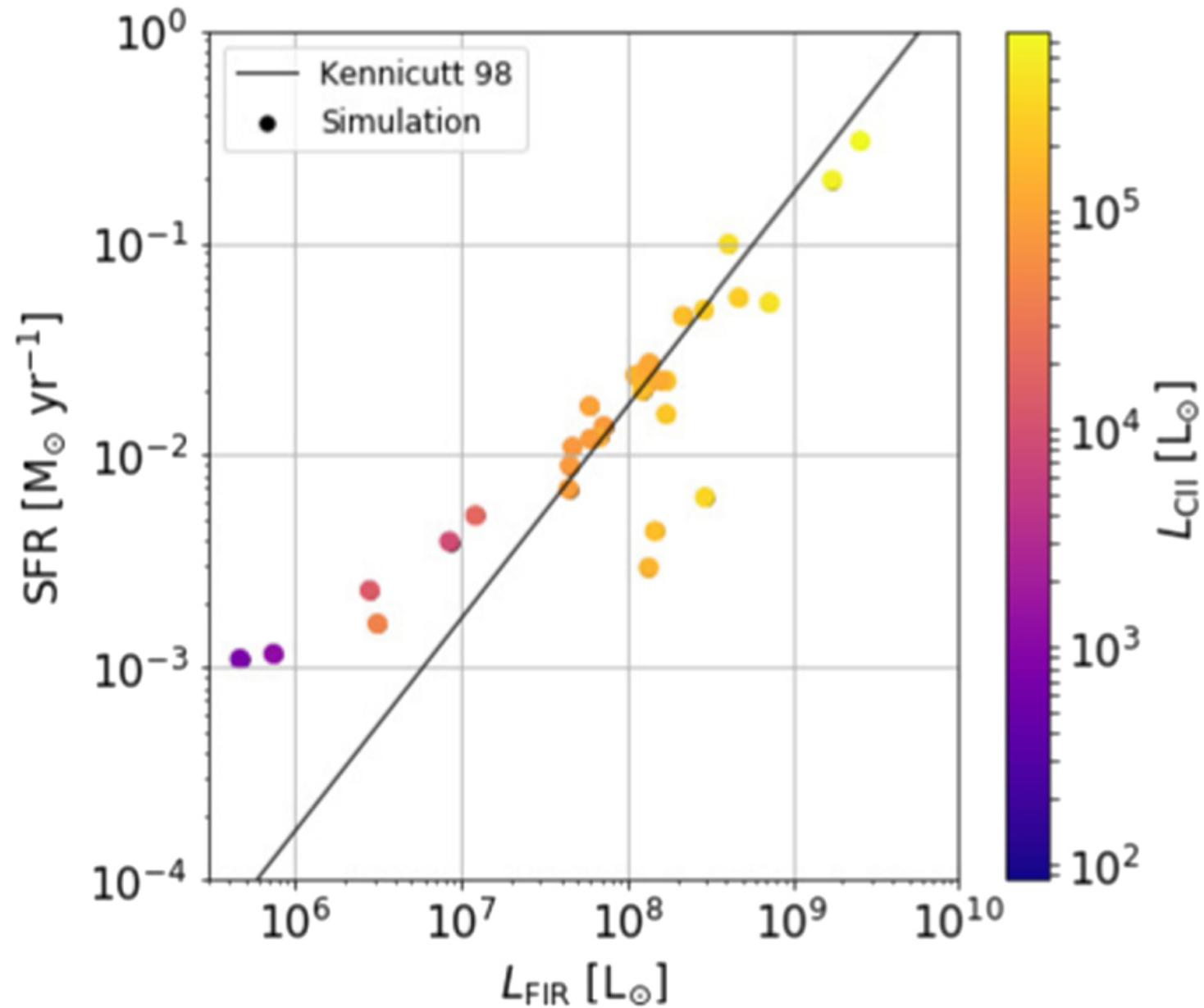
Figure 12. from Thomas G. Bisbas et al 2022 Astrophys. J. 934 doi:10.3847/1538-4357/ac7960 https://dx.doi.org/10.3847/1538-4357/ac7960 © 2022. The Author(s). Published by the American Astronomical Society.
