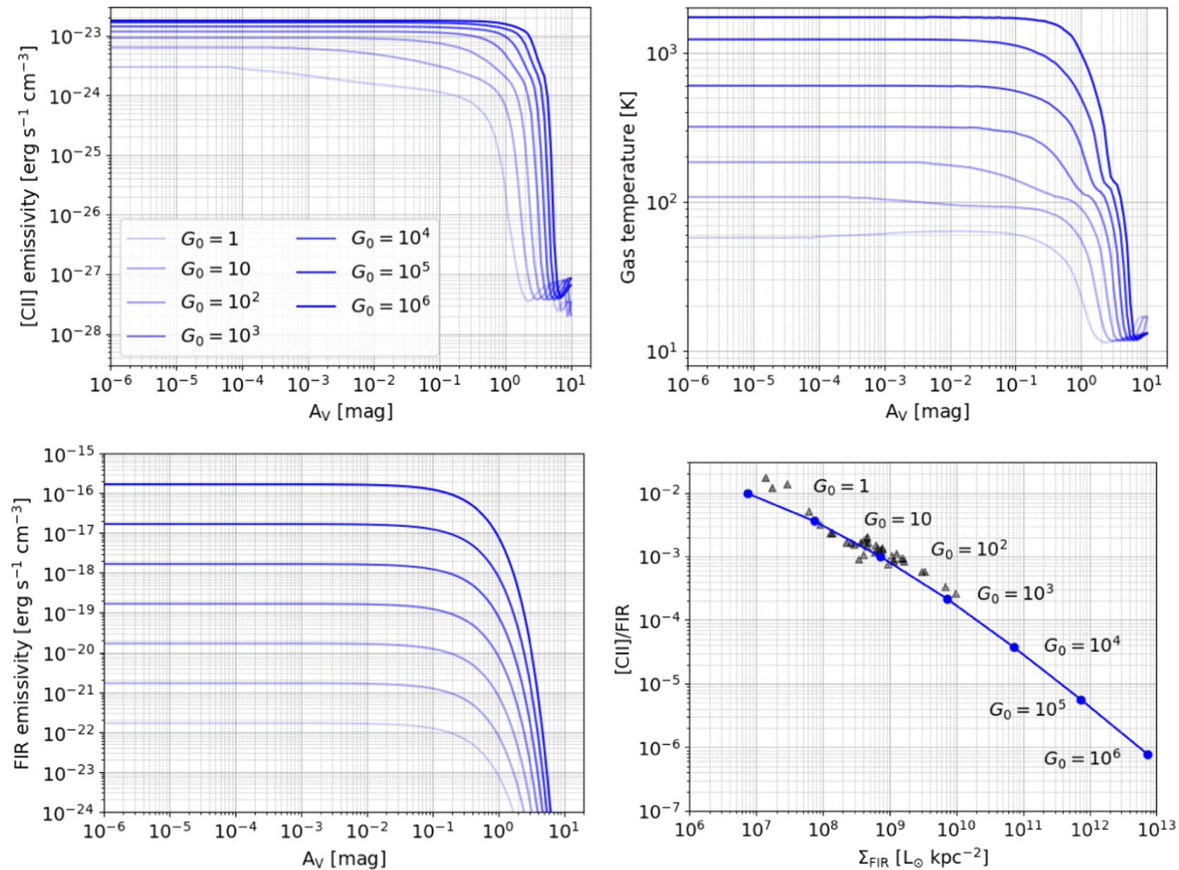
Figure 11. from Thomas G. Bisbas et al 2022 Astrophys. J. 934 doi:10.3847/1538-4357/ac7960 https://dx.doi.org/10.3847/1538-4357/ac7960 © 2022. The Author(s). Published by the American Astronomical Society.
