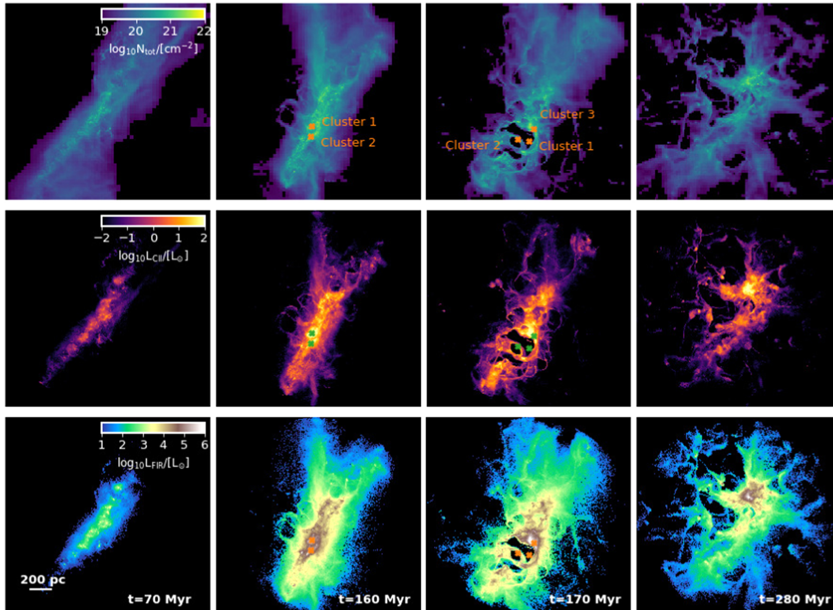
Figure 1. from Thomas G. Bisbas et al 2022 Astrophys. J. 934 doi:10.3847/1538-4357/ac7960 https://dx.doi.org/10.3847/1538-4357/ac7960 © 2022. The Author(s). Published by the American Astronomical Society.
