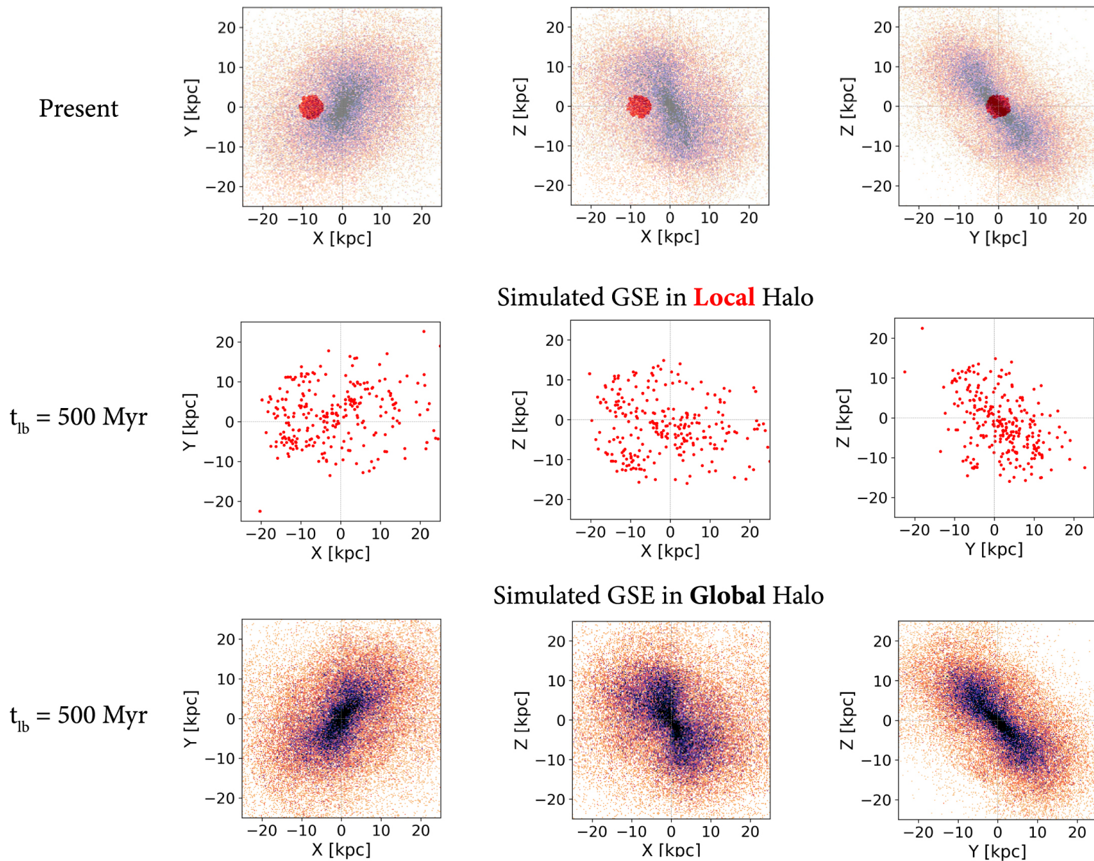
Figure 7. from Jiwon Jesse Han et al 2022 Astrophys. J. 934 doi:10.3847/1538-4357/ac795f https://dx.doi.org/10.3847/1538-4357/ac795f © 2022. The Author(s). Published by the American Astronomical Society.
