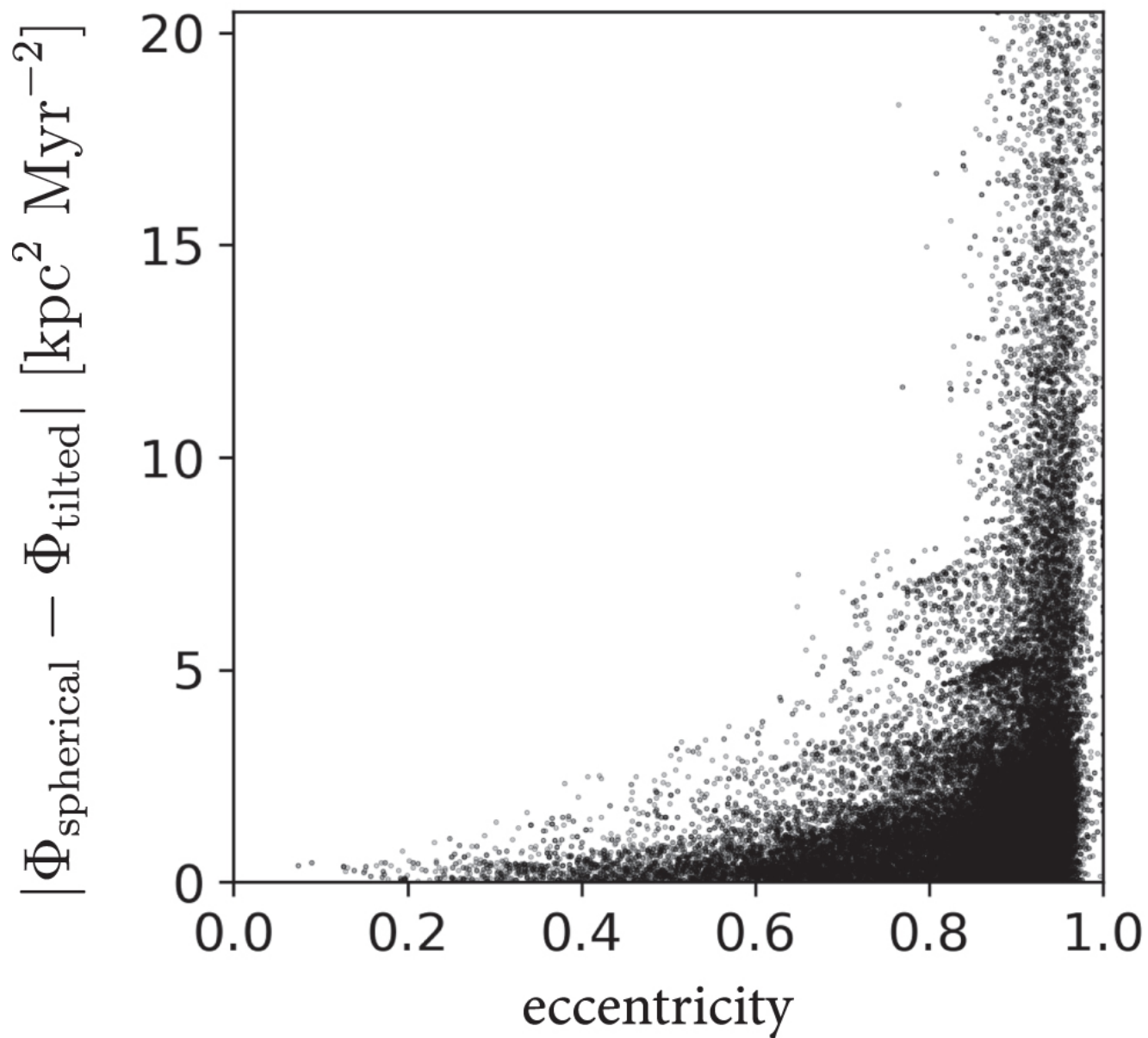
Figure 6. from Jiwon Jesse Han et al 2022 Astrophys. J. 934 doi:10.3847/1538-4357/ac795f https://dx.doi.org/10.3847/1538-4357/ac795f © 2022. The Author(s). Published by the American Astronomical Society.
