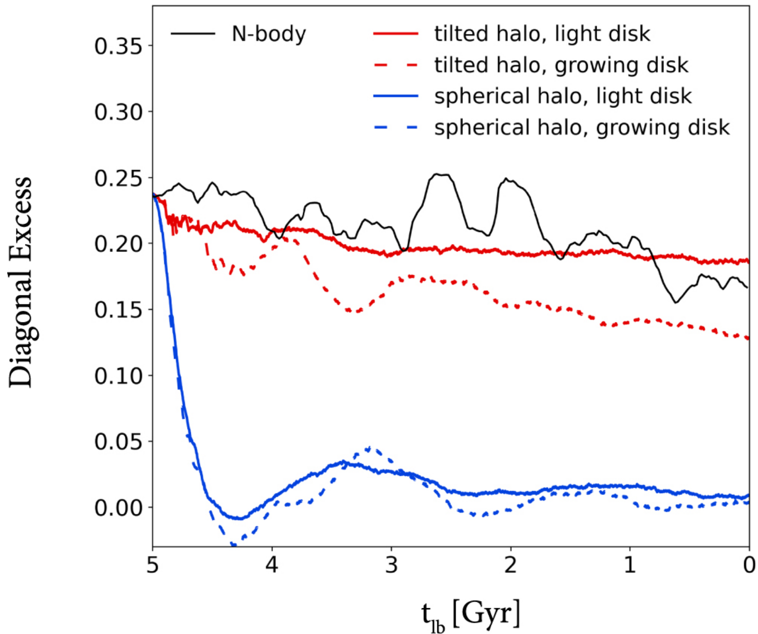
Figure 5. from Jiwon Jesse Han et al 2022 Astrophys. J. 934 doi:10.3847/1538-4357/ac795f https://dx.doi.org/10.3847/1538-4357/ac795f © 2022. The Author(s). Published by the American Astronomical Society.
