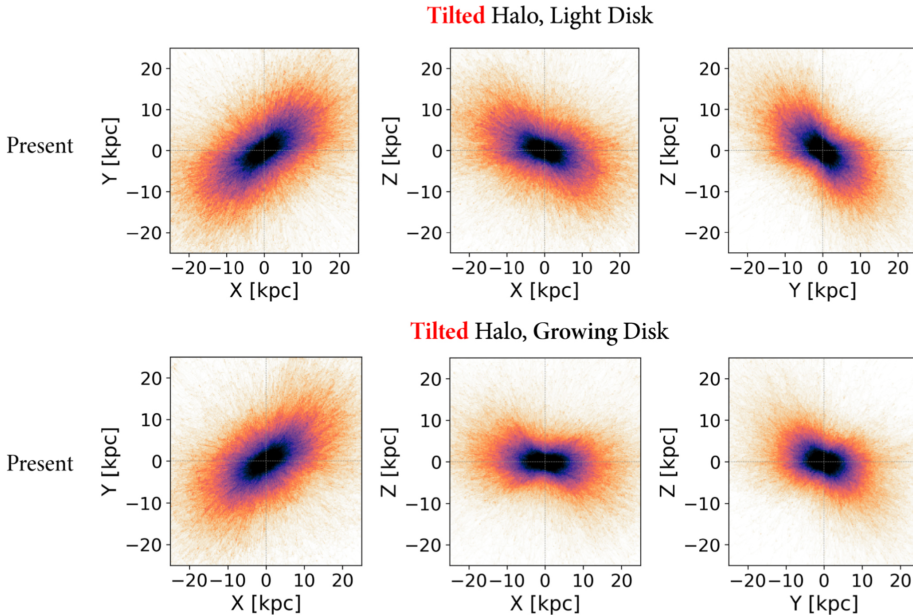
Figure 4. from Jiwon Jesse Han et al 2022 Astrophys. J. 934 doi:10.3847/1538-4357/ac795f https://dx.doi.org/10.3847/1538-4357/ac795f © 2022. The Author(s). Published by the American Astronomical Society.
