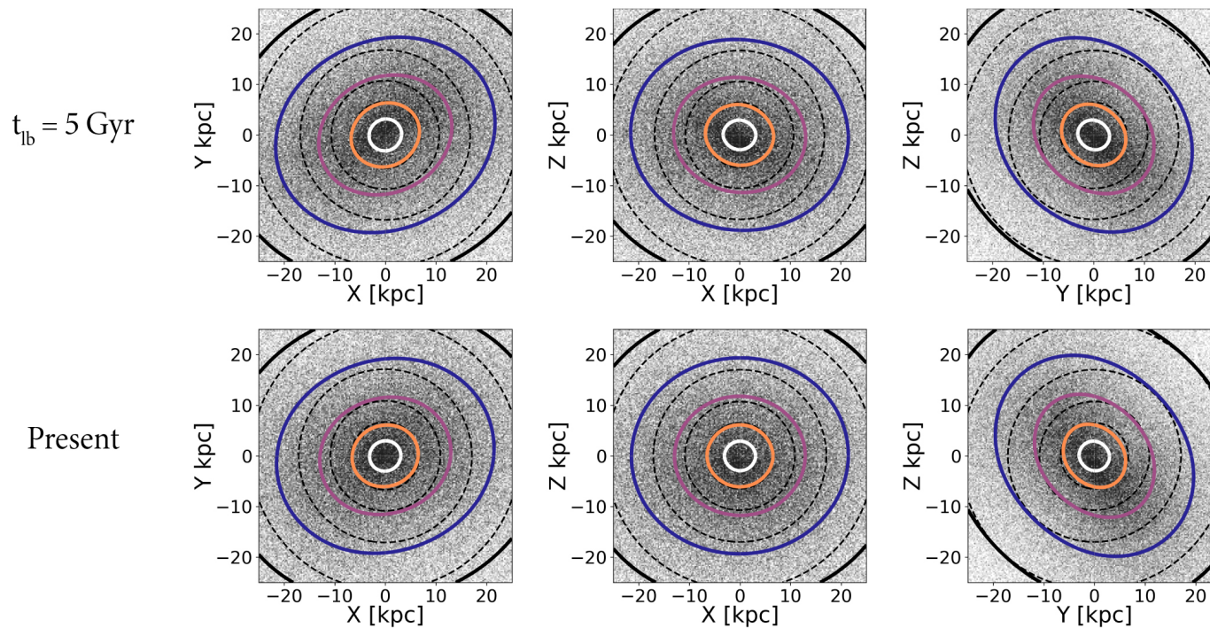
Figure 1. from Jiwon Jesse Han et al 2022 Astrophys. J. 934 doi:10.3847/1538-4357/ac795f https://dx.doi.org/10.3847/1538-4357/ac795f © 2022. The Author(s). Published by the American Astronomical Society.
