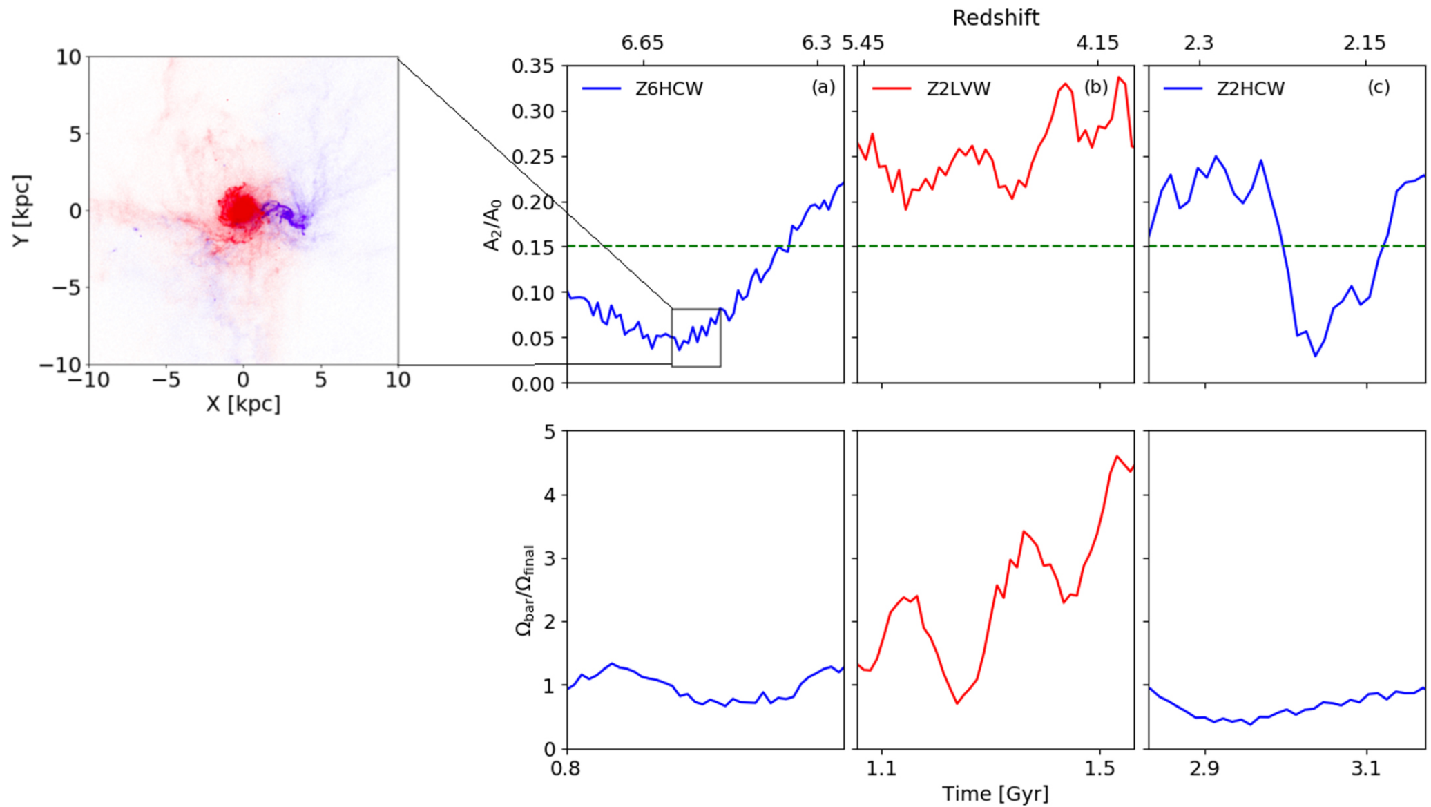
Figure 8. from Da Bi et al 2022 Astrophys. J. 934 doi:10.3847/1538-4357/ac779b https://dx.doi.org/10.3847/1538-4357/ac779b © 2022. The Author(s). Published by the American Astronomical Society.
