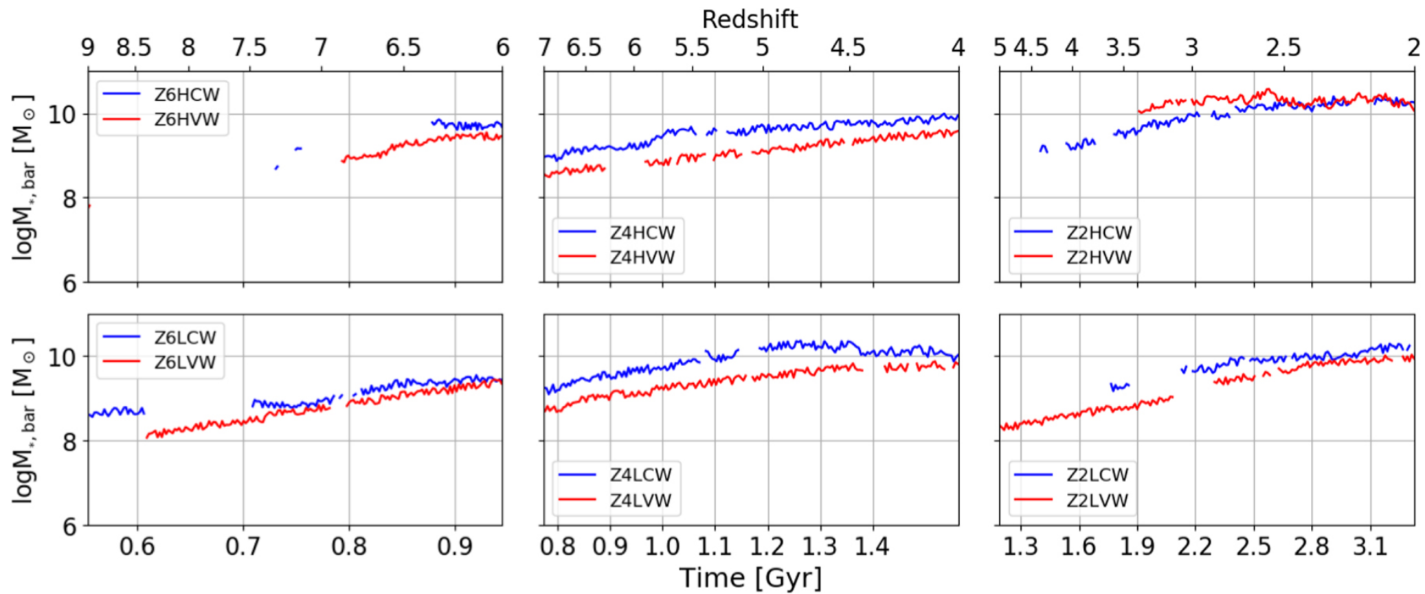
Figure 4. from Da Bi et al 2022 Astrophys. J. 934 doi:10.3847/1538-4357/ac779b https://dx.doi.org/10.3847/1538-4357/ac779b © 2022. The Author(s). Published by the American Astronomical Society.
