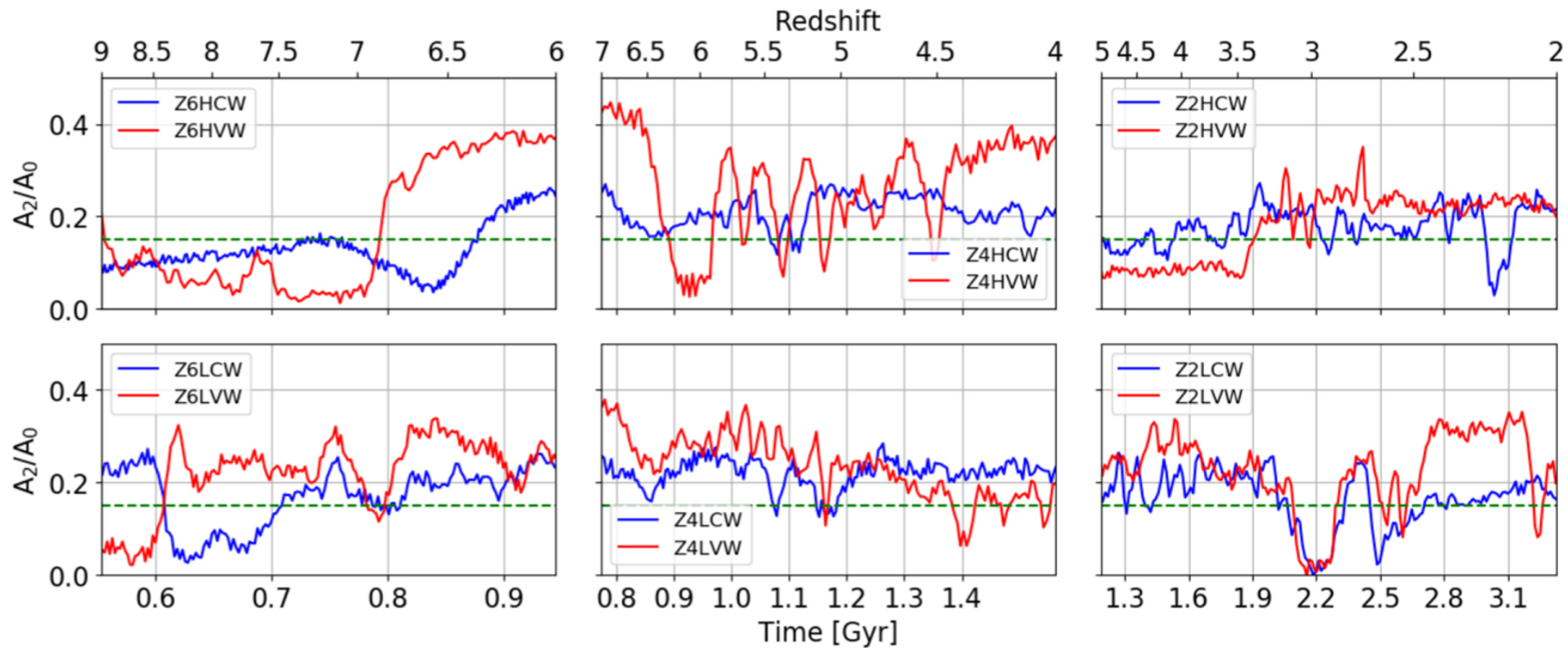
Figure 3. from Da Bi et al 2022 Astrophys. J. 934 doi:10.3847/1538-4357/ac779b https://dx.doi.org/10.3847/1538-4357/ac779b © 2022. The Author(s). Published by the American Astronomical Society.
