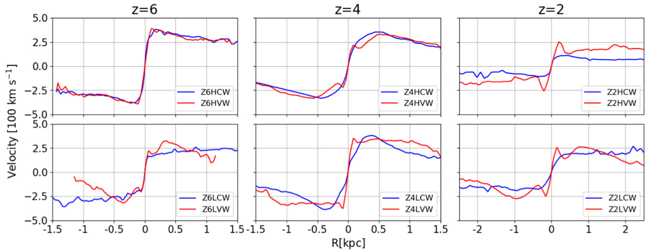
Figure 2. from Da Bi et al 2022 Astrophys. J. 934 doi:10.3847/1538-4357/ac779b https://dx.doi.org/10.3847/1538-4357/ac779b © 2022. The Author(s). Published by the American Astronomical Society.
