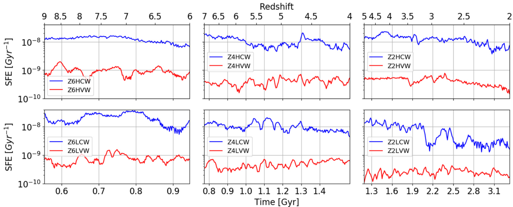
Figure 15. from Da Bi et al 2022 Astrophys. J. 934 doi:10.3847/1538-4357/ac779b https://dx.doi.org/10.3847/1538-4357/ac779b © 2022. The Author(s). Published by the American Astronomical Society.
