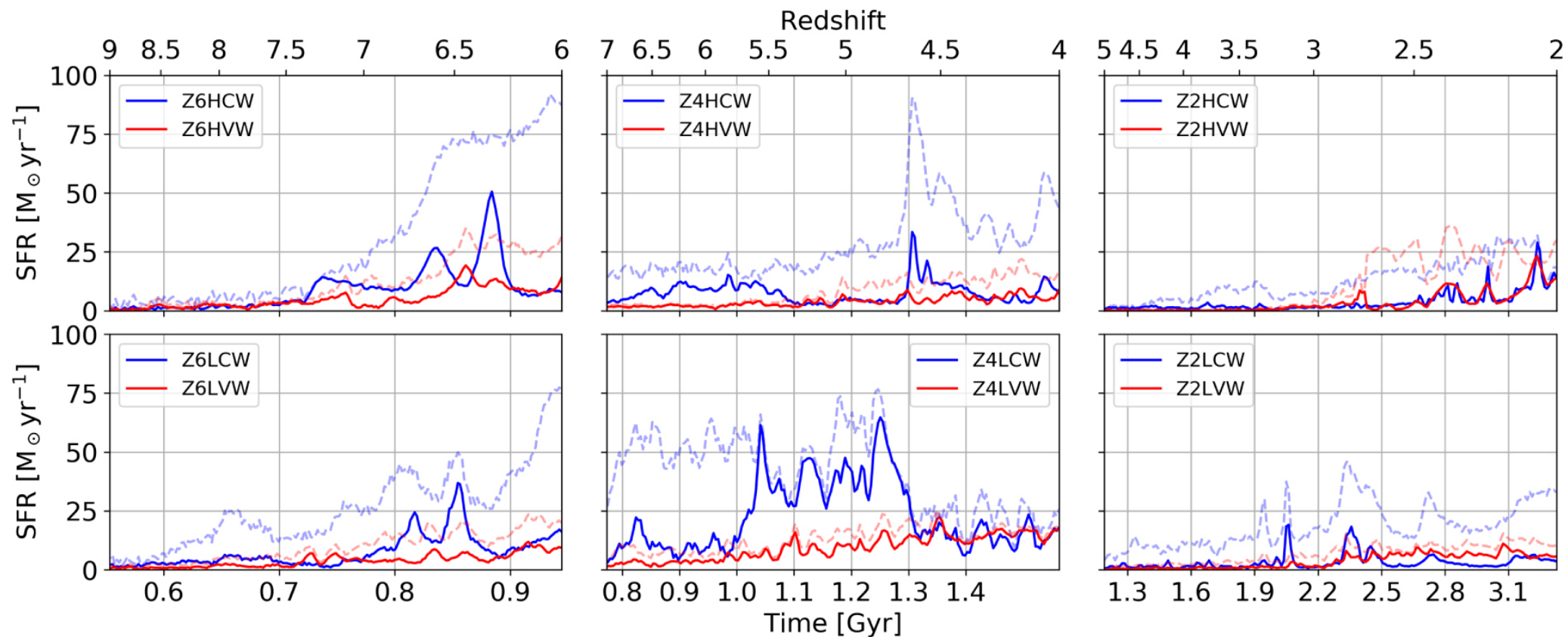
Figure 13. from Da Bi et al 2022 Astrophys. J. 934 doi:10.3847/1538-4357/ac779b https://dx.doi.org/10.3847/1538-4357/ac779b © 2022. The Author(s). Published by the American Astronomical Society.
