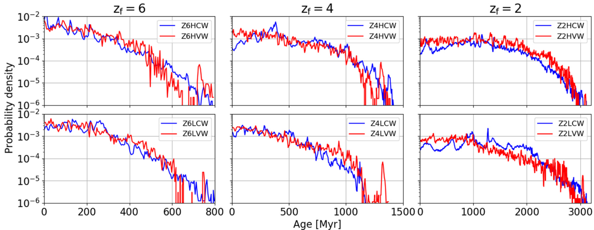
Figure 12. from Da Bi et al 2022 Astrophys. J. 934 doi:10.3847/1538-4357/ac779b https://dx.doi.org/10.3847/1538-4357/ac779b © 2022. The Author(s). Published by the American Astronomical Society.
