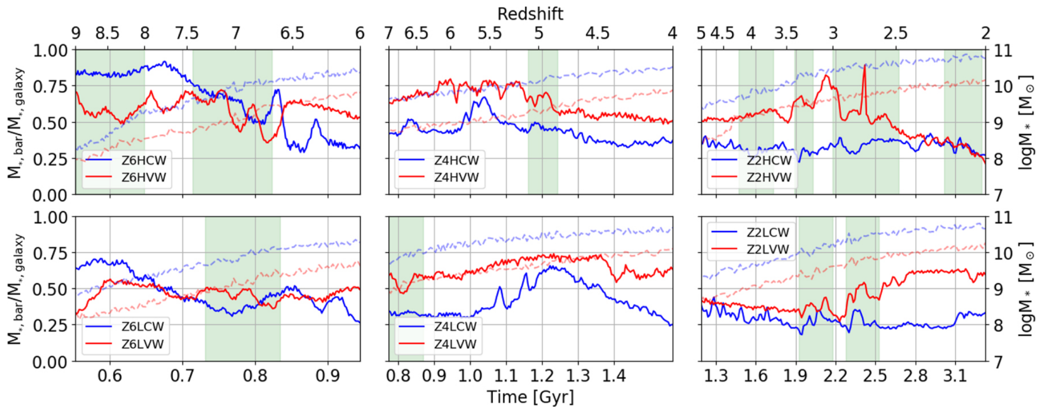
Figure 1. from Da Bi et al 2022 Astrophys. J. 934 doi:10.3847/1538-4357/ac779b https://dx.doi.org/10.3847/1538-4357/ac779b © 2022. The Author(s). Published by the American Astronomical Society.
