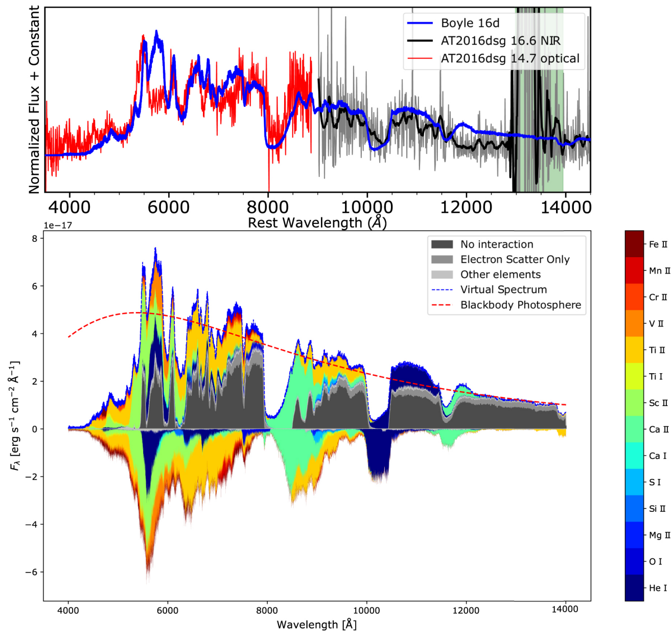
Figure 8. from Yize Dong et al 2022 Astrophys. J. 934 doi:10.3847/1538-4357/ac75eb https://dx.doi.org/10.3847/1538-4357/ac75eb © 2022. The Author(s). Published by the American Astronomical Society.
