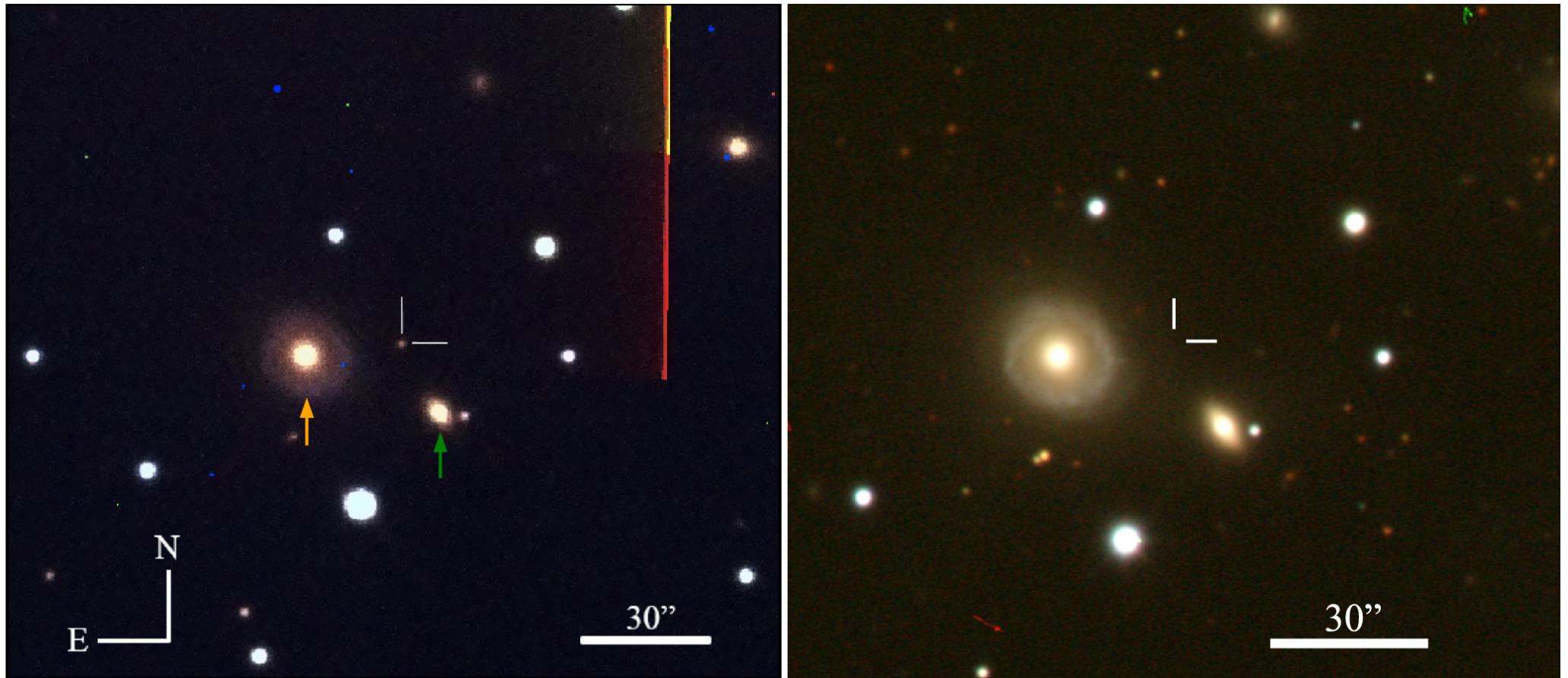
Figure 1. from Yize Dong et al 2022 Astrophys. J. 934 doi:10.3847/1538-4357/ac75eb https://dx.doi.org/10.3847/1538-4357/ac75eb © 2022. The Author(s). Published by the American Astronomical Society.
